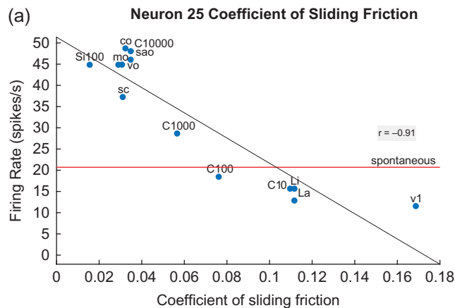
Figure 1. An orbitofrontal taste cortex neuron with responses linearly correlated with decreases in the CSF (a). Low CSFs indicate lubricity produced, for example, by the oils. The linear regression line shown has a correlation of r = -0.91 ( P = 1.2 \times 10^{-5} ) between the firing rate of the neuron and the CSF. The closeness of the data points to this regression line and the value of the correlation coefficient indicate how well the data fit a linear function of the CSF. (b): There is a much weaker relation to viscosity ( r = 0.68 , P = 0.01 ), with the oils producing a larger response than predicted linearly. Further, a regression line through the nonoil stimuli would have a much lower slope. C10–C10000: carboxymethylcellulose with the nominal viscosity of 10, 100, 1000 and 10000 cP. v1: water (1 cP). co: coconut oil; mo: mineral oil; sao: safflower oil; vo: vegetable oil; sc: single cream. Si10, Si100, Si1000: silicone oil with the viscosity indicated. LiA: linoleic acid; LaA: lauric acid. The horizontal line indicates the spontaneous firing rate. The Pearson correlation between the firing rate of each neuron and (a) the CSF, and (b) the viscosity was calculated to show to what extent the firing of a neuron reflected one or other of these measures. Linear regression lines are shown in the figures for how the firing rates were related to the CSF, or to the log of the viscosity. (The log of the viscosity was used because human psychophysical measures of the thickness of these stimuli were linearly related to the log of the viscosity (Kadohisa et al. 2005a).) Each firing rate value shown in the Figure and used in the statistical analyses presented in detail in the Supplementary Material is the mean of four or more firing rate measurements taken in random permuted sequence across the set of stimuli, with standard errors shown in the original publications (Verhagen et al. 2003, 2004; Kadohisa et al. 2005a; 2005b). Moreover, it has been established that some cortical neurons respond to water in the mouth; and that some neurons can respond to oral stimuli by decreasing their firing rates below the spontaneous level of firing (Scott et al. 1986; Rolls et al. 1990; Yaxley et al. 1990; Verhagen et al. 2003, 2004; Kadohisa et al. 2005a, 2005b).
