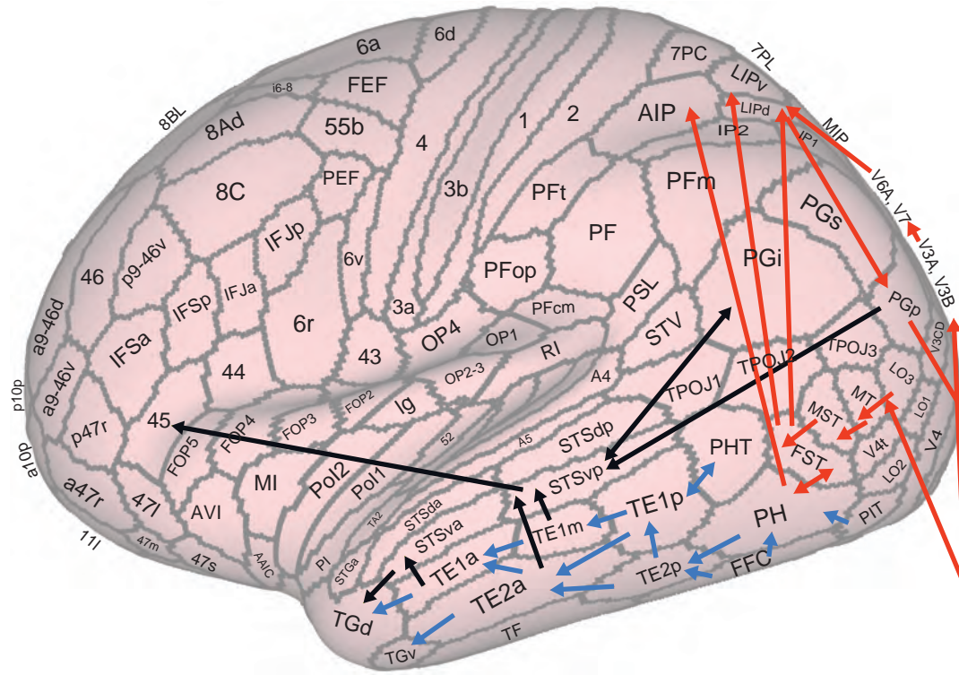
HCP-MMP human brain cortical visual streams: lateral view
