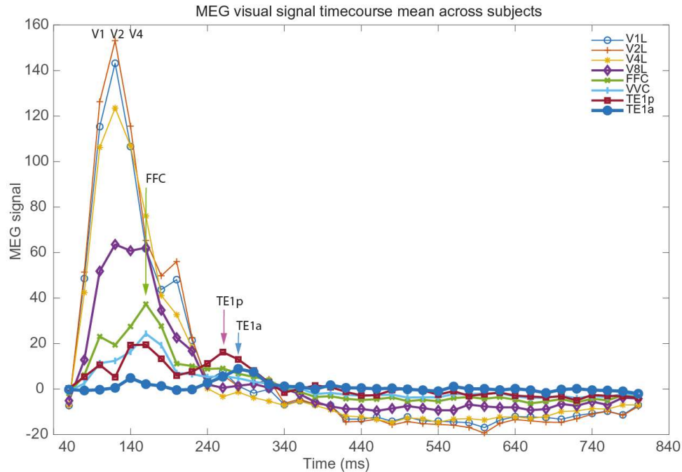
Fig. S2. The timecourse of the MEG signal in different HCP-MMP ventral visual stream cortical regions. The onset of the face or tool visual stimuli was at time 0. The amplitude of the MEG signal for the the face, tool, 0-back and 2-back conditions was averaged across 83 participants. V1, V2, and V4 are early visual cortical regions. V8 is just before the fusiform face cortex, FFC. The ventral visual complex VVC probably receives from V8, is medial to the FFC (Fig. 1), is part of a route for visual information from visual cortical regions to reach the hippocampus, and is part of / leads to the parahippocampal scene (or place) area (Rolls et al., 2023a). TE1p is an example of an inferior temporal cortex visual region. TE1a is an example of an anterior inferior temporal cortex region involved in semantic representations (Rolls et al., 2022a, 2023a). The results are for the left hemisphere. The duration of the response may be short because fixation on the stimuli may be for only a short time period. (After Rolls et al., 2023c) (VisMEGtimecourse31.eps).
