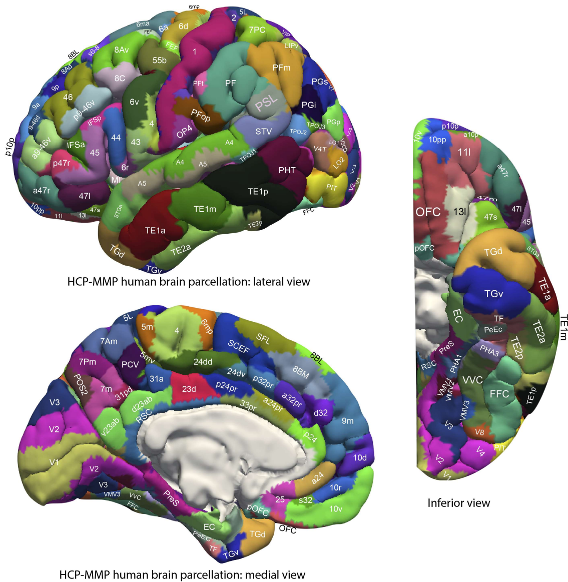
Fig. S1-5. Anatomical regions of the human visual and other cortical regions. Regions are shown as defined in the HCP-MMP atlas (Glasser et al., 2016), and in its extended version HCPex (Huang et al., 2022). The regions are shown on images of the human brain without the sulci expanded to show which cortical HCP-MMP regions are normally visible, for comparison with Figs. 6-10. (The ICBM153 MNI T1 image was used to prepare this figure.) Abbreviations are provided in Table S1.
