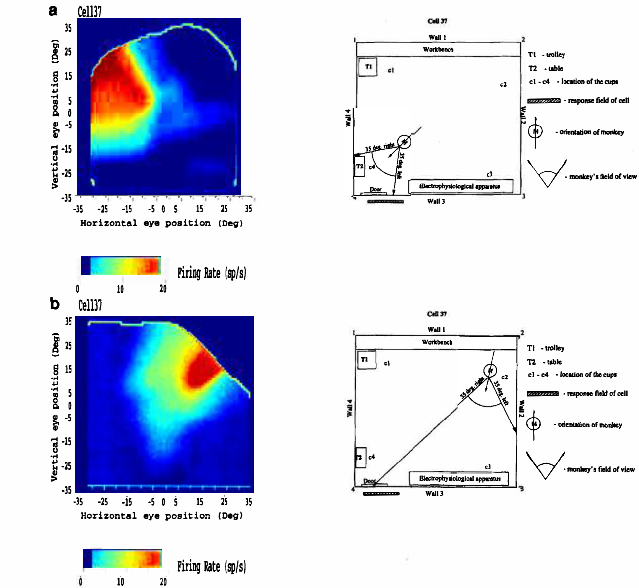
FIG. 2. (a) The firing rate of a spatial view cell (cell 37 in Table 1 and Fig. 3) with the monkey stationary in the environment, with its head direction indicated by the arrow and moving its eyes to look at different parts of the environment. (b) Similar data when the monkey was at a different place in the environment and with a different head direction. The cell increased its firing rate when the monkey looked at some parts of the environment (e.g. towards corner 4). The firing rate of the cell in spikes/s is indicated by the blackness of the diagram on the left. Calibration bar in spikes/s is shown below. The field of view sampled by the monkey is shown by the part of the firing rate greyscale plot that is contained by the black perimeter line. (c) A summary of the firing rates when the monkey was looking at different spatial views in the environment, from different places and with different head directions. The acute angle of the solid triangle indicates the head direction. The short lines within the circle indicate the view directions (binned with 17.5 degrees per bin) in which data were available. The bars outside the circle represent the mean firing rate (and the SEM) of the cell when the monkey was looking in that direction; the absence of a bar outside the circle where data were available indicates a firing rate of 0 spikes/s.
